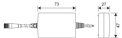
Mains PSU
