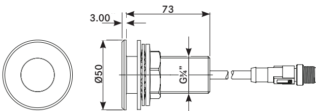
Programmable WC Sensor
