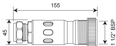
Air Break For Direct Flushing
